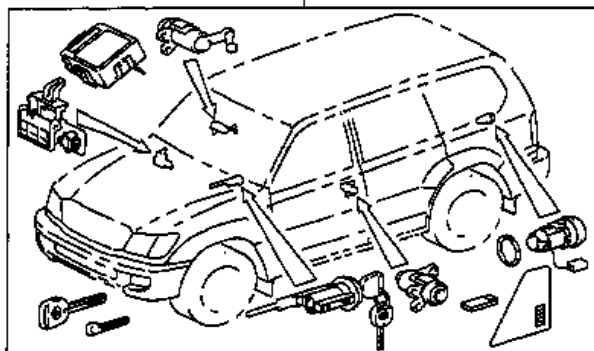
① TRANSMITTER
