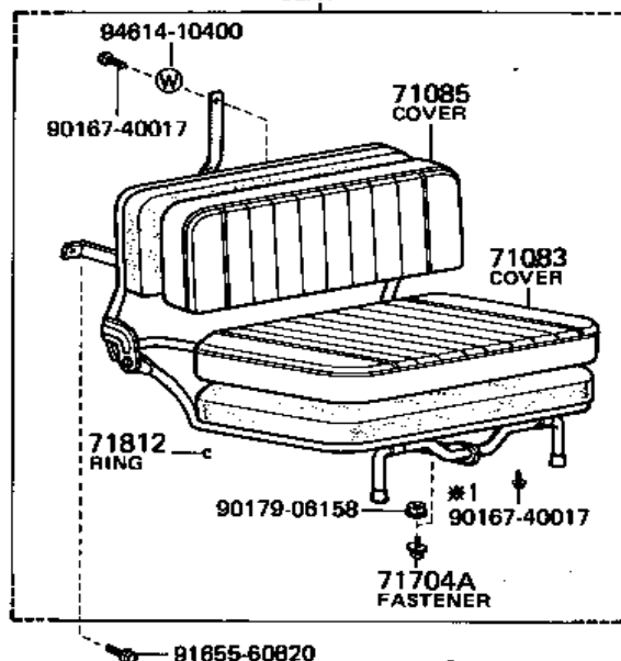
71700 SEAT
