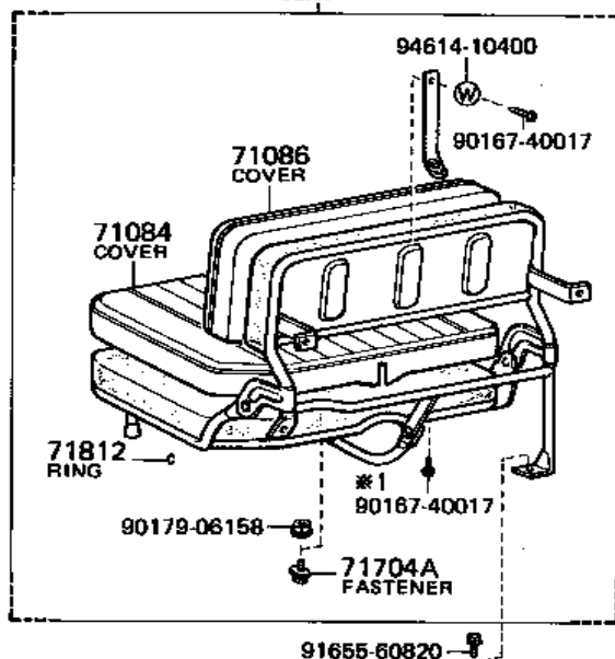
71800 SEAT
